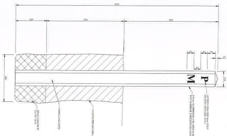
PIPELINE PRECAST CONCRETE MARKER BEACON 1:75
