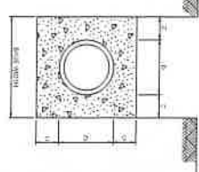
DETAIL OF CONCRETE ENCASEMENT
