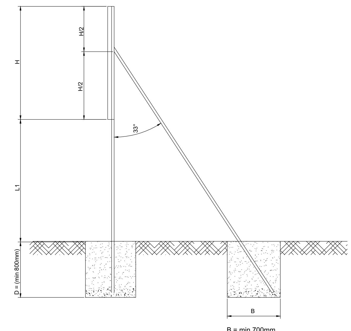
SIDE ELEVATION
