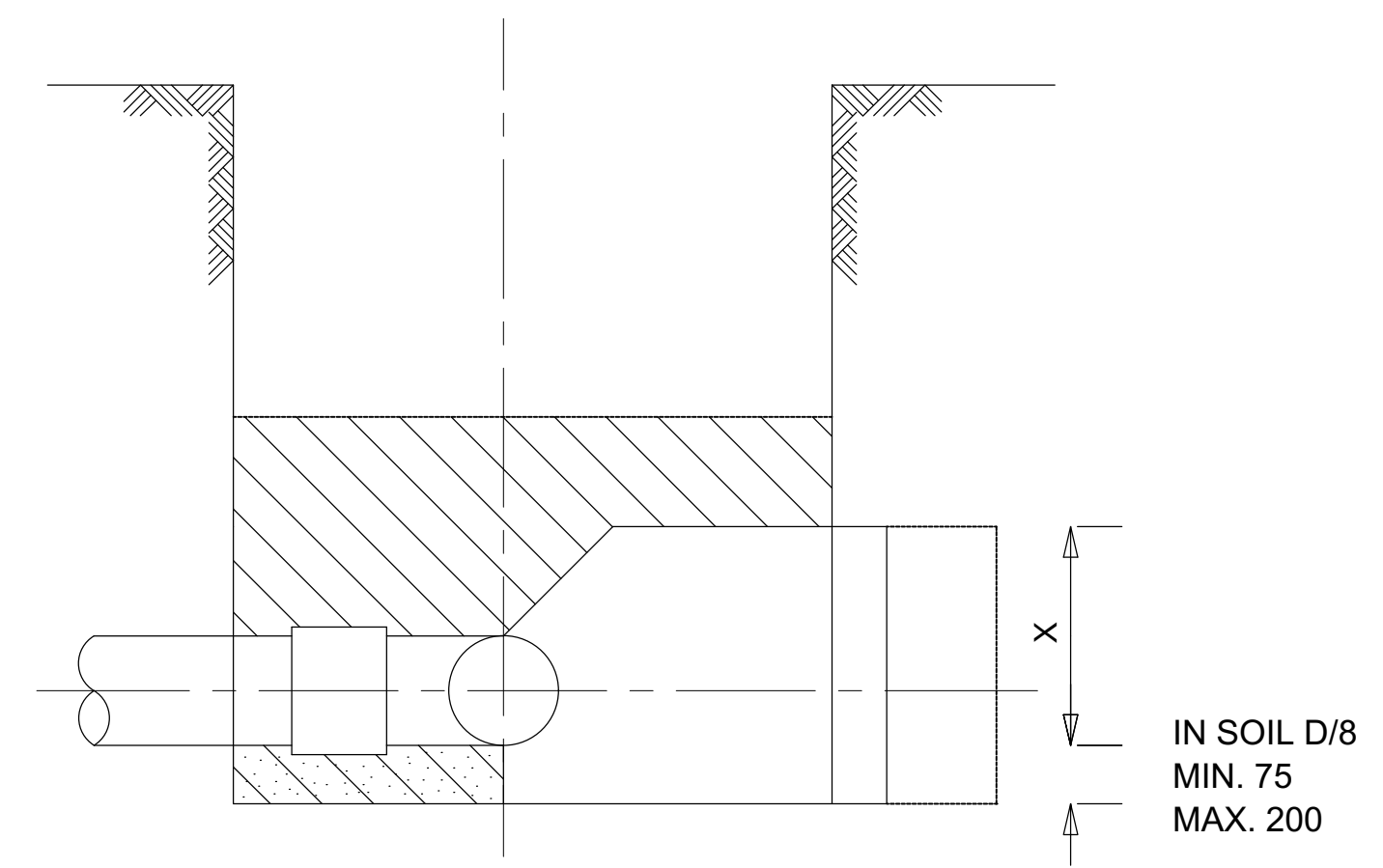
ELEVATION "A"
