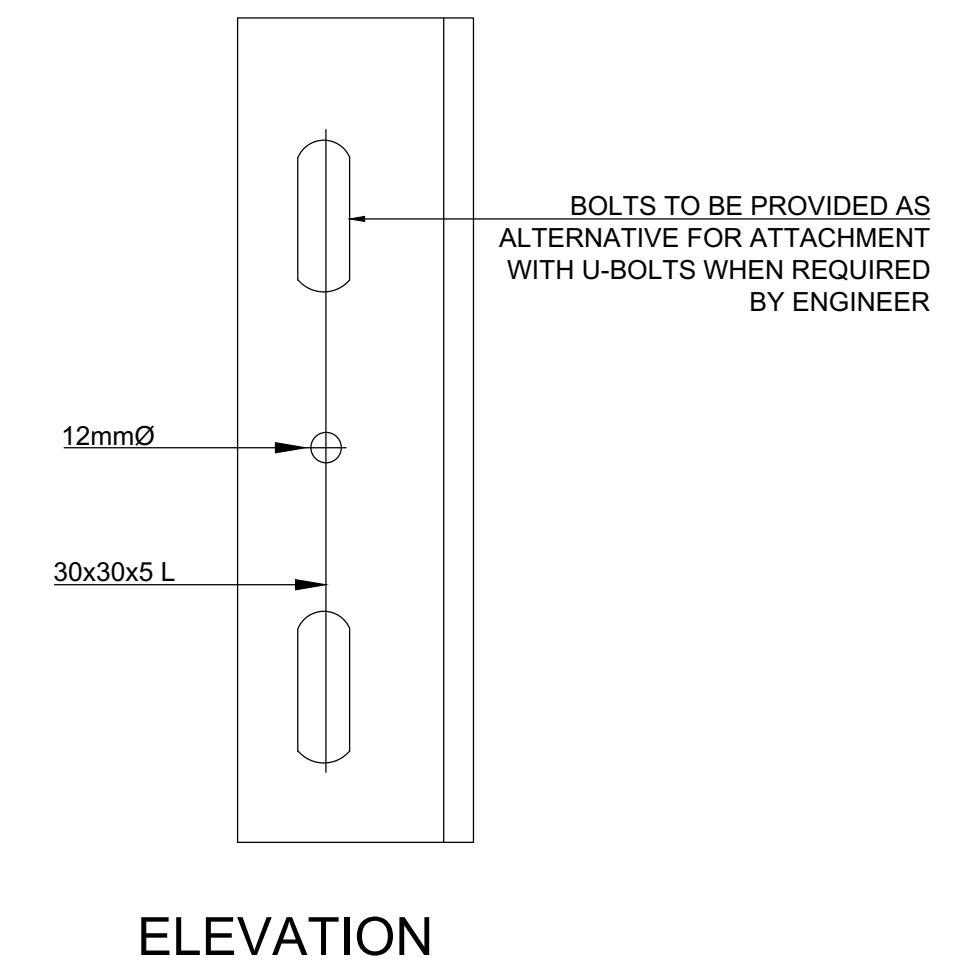
ERECTION BRACKET
