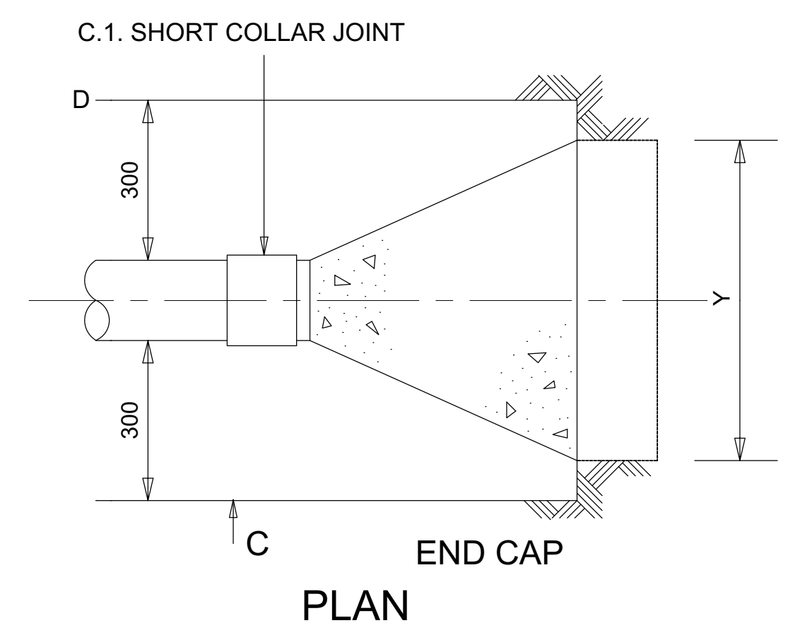
PLAN
