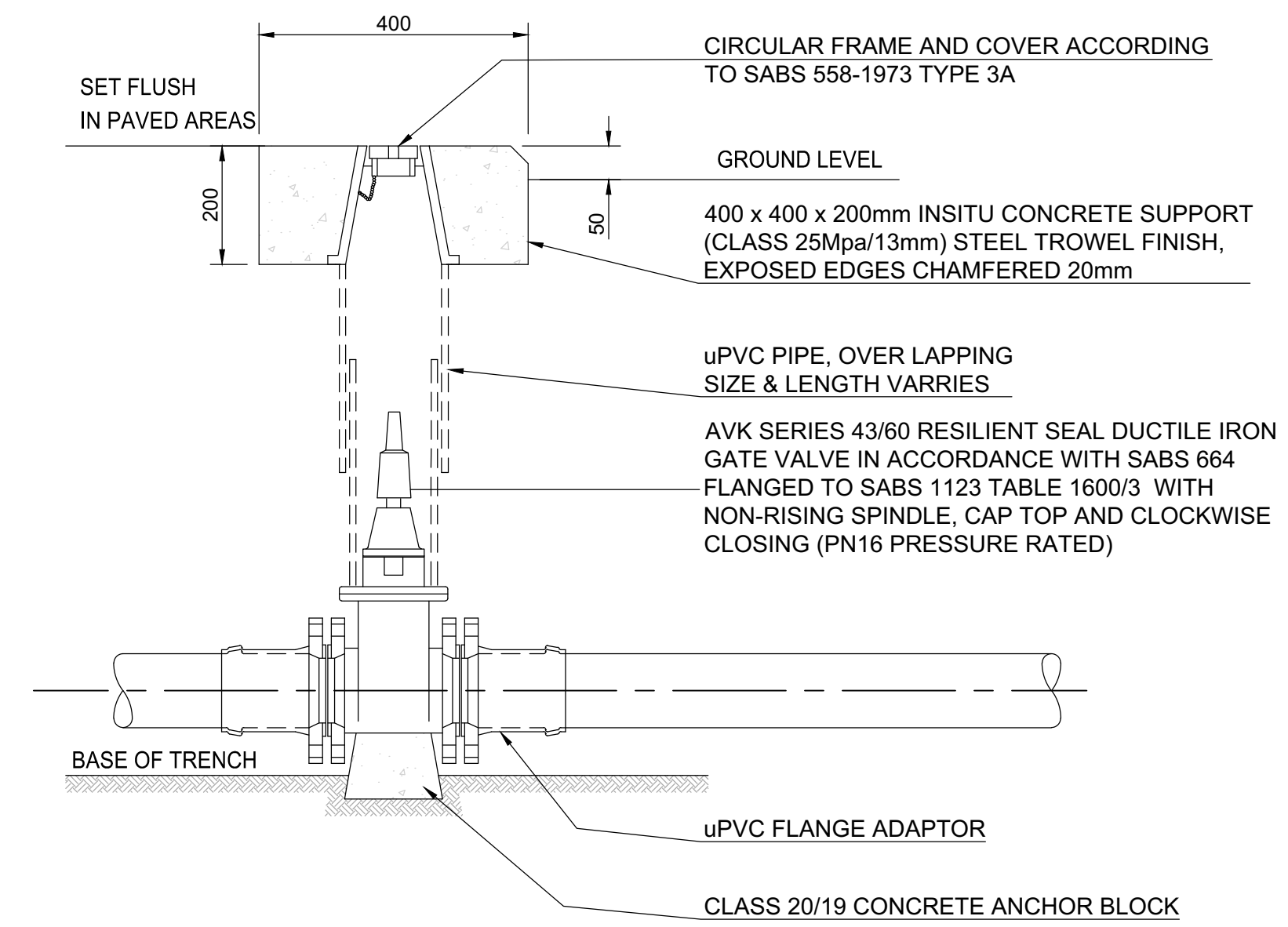
WATER LINE ISOLATING VALVE (50-160mmØ) SCALE 1 : 10
