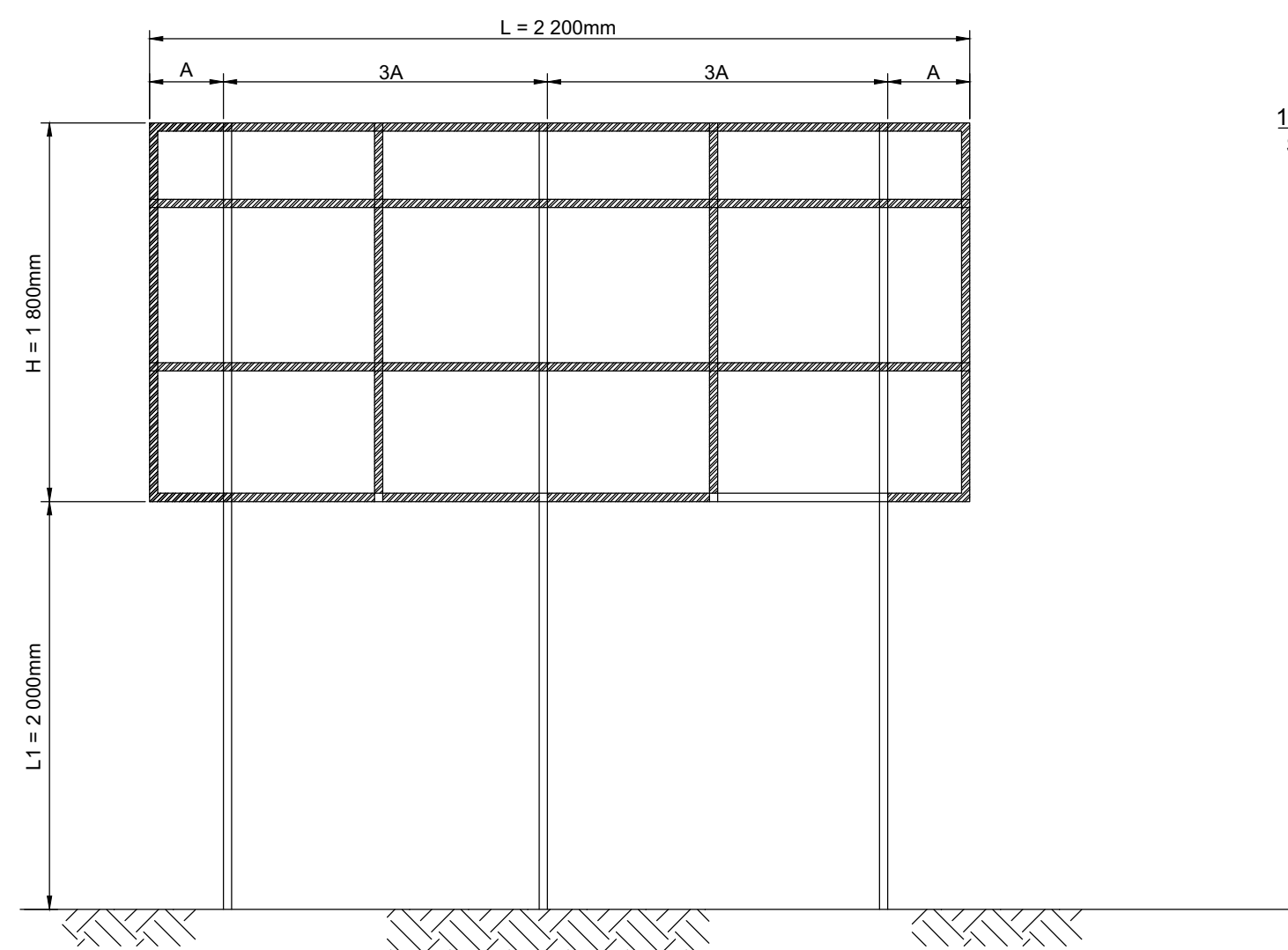
BACK ELEVATION
