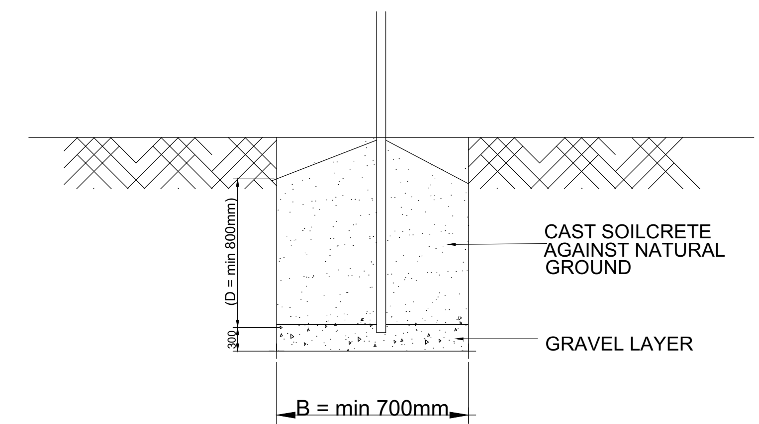
FOUNDATION DETAIL
