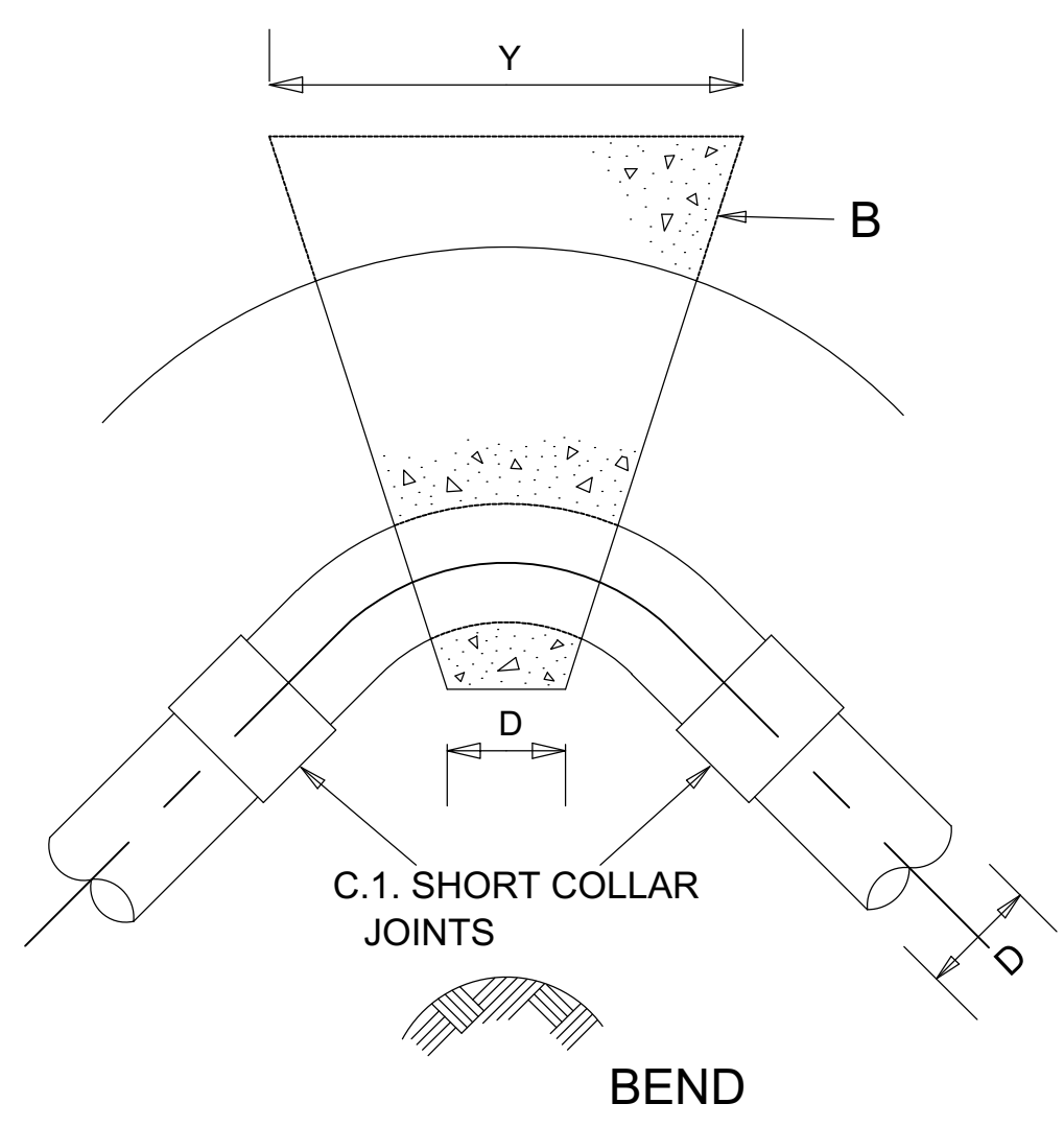
PLAN
