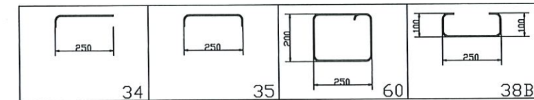
81kL ELEVATED TANK ON 8m STAND BENDING SCHEDULE FOR 04 FOOTINGS
