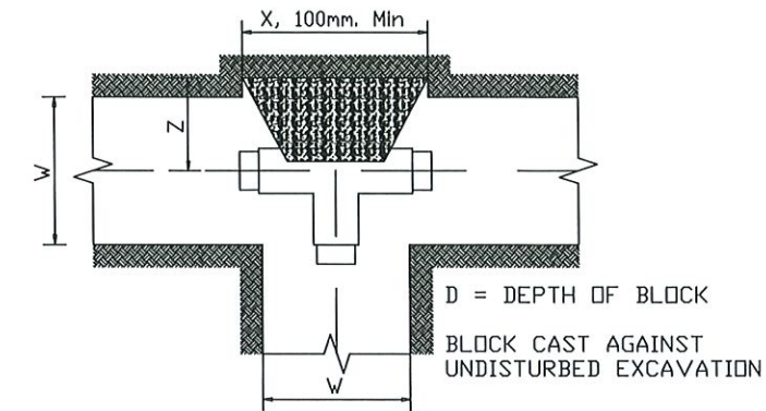
THRUST BLOCK FOR TEE
