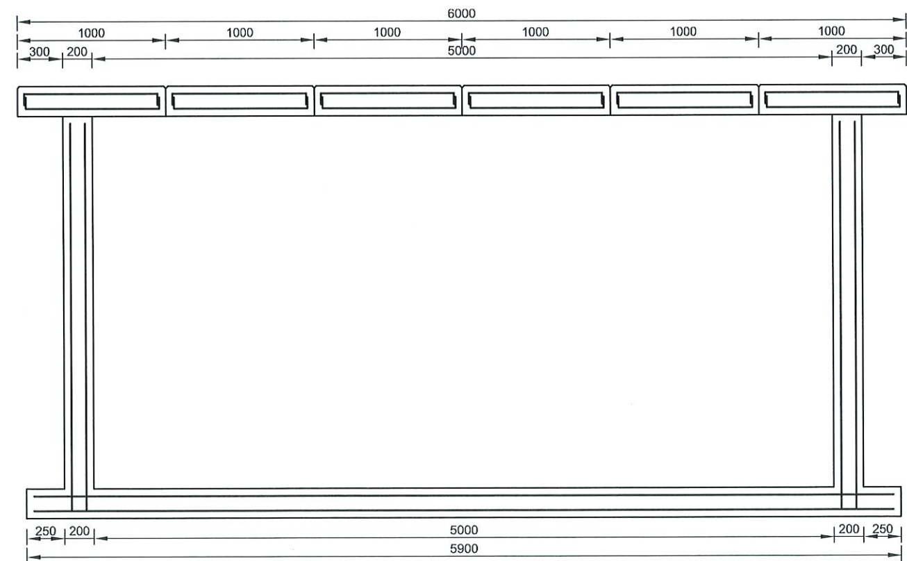
5m VALVE CHAMBER REINFORCEMENT
