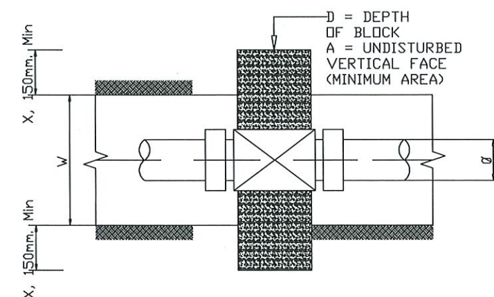
THRUST BLOCK FOR GATE VALVE
