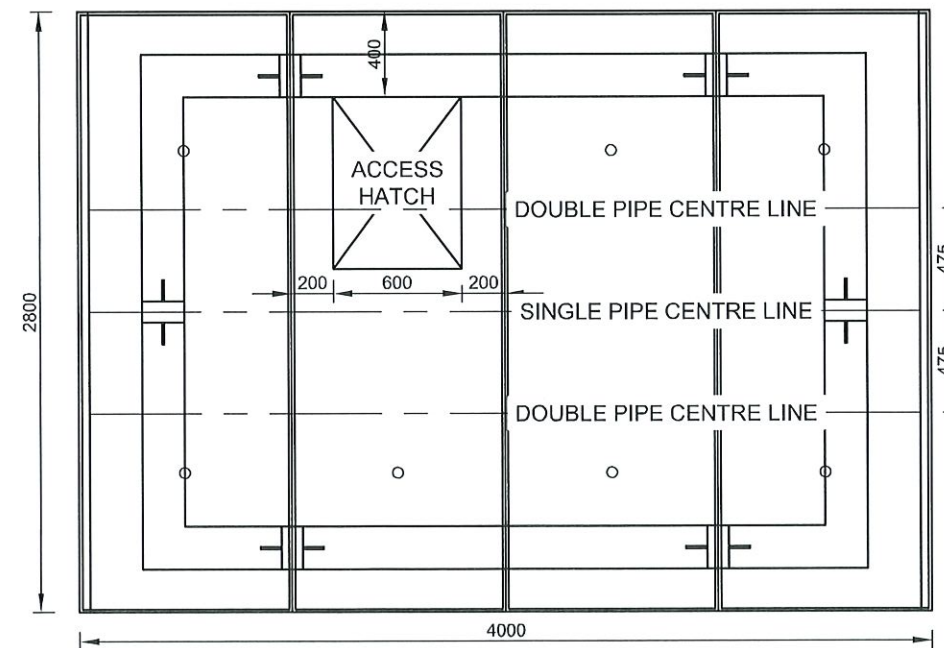
VALVE CHAMBER TYPICAL PLAN
