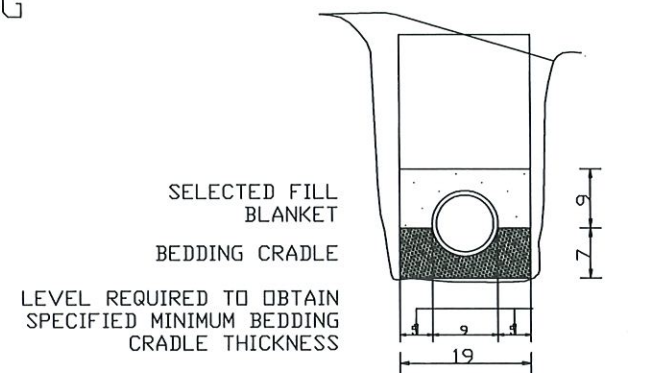
MEASUREMENT OF BEDDING N.T.S
