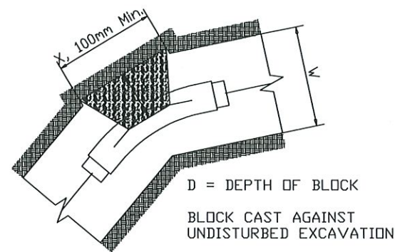
THRUST BLOCK FOR 45° BEND
