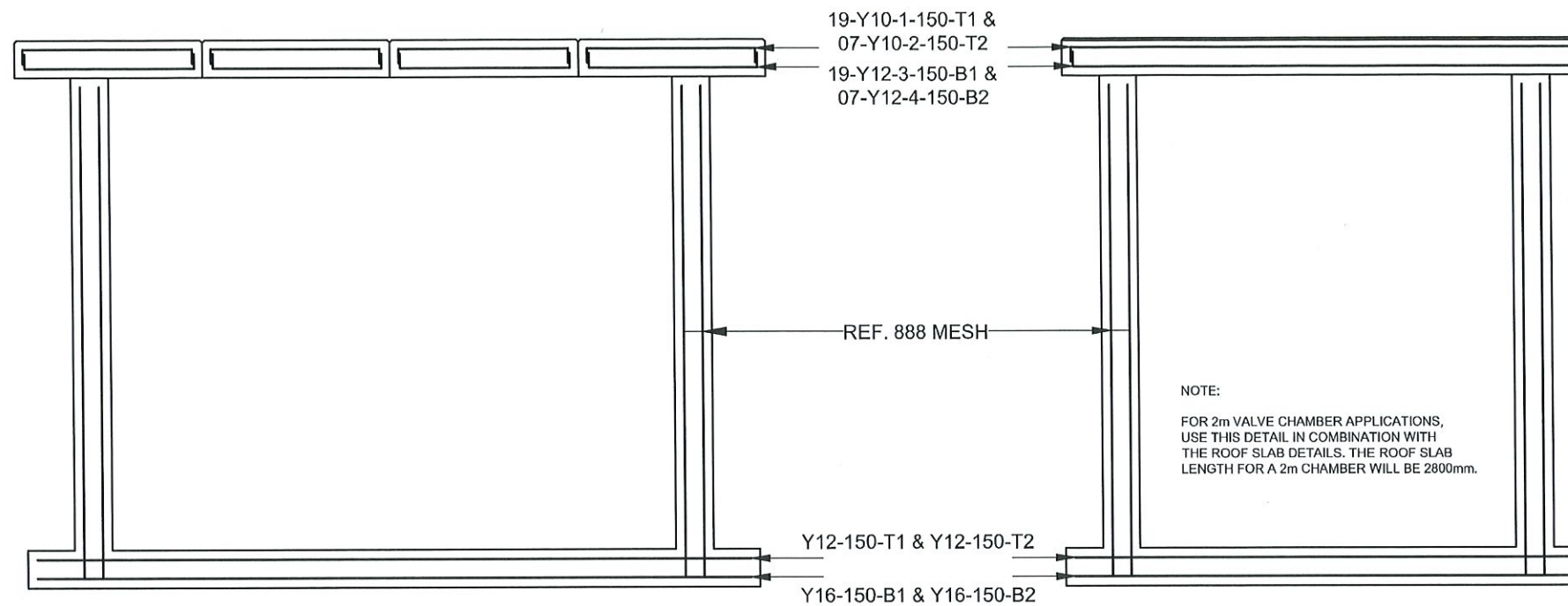
3m VALVE CHAMBER REINFORCEMENT
