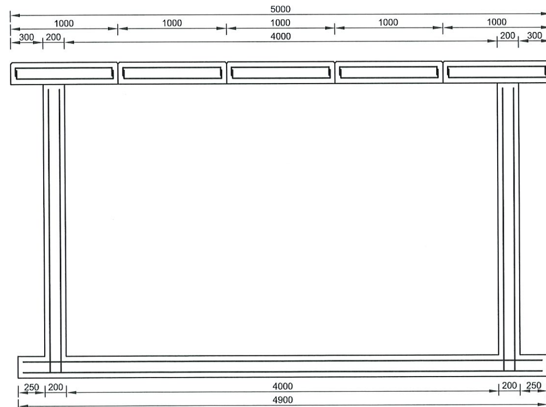
4m VALVE CHAMBER REINFORCEMENT
