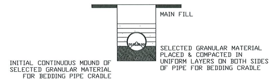
FLEXIBLE PIPE SUPPORTED ON SELECTED GRANULAR MATERIAL CONSTRUCTION METHOD OF PIPE BEDDING N.T.S
