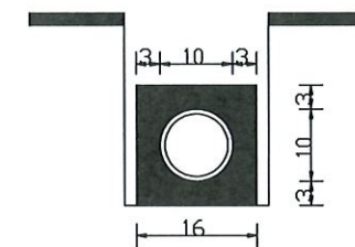
DETAIL OF CONCRETE ENCASEMENT N.T.S
