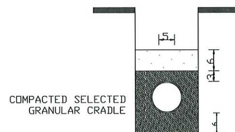
FLEXIBLE PIPE SUPPORTED ON SELECTED GRANULAR MATERIAL DETAIL OF PIPE BEDDING N.T.S
