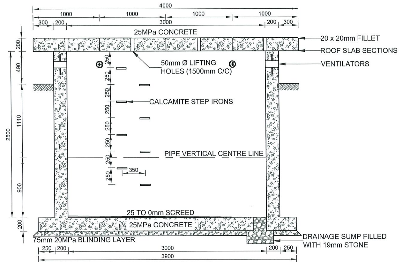
VALVE CHAMBER TYPICAL ELEVATION
