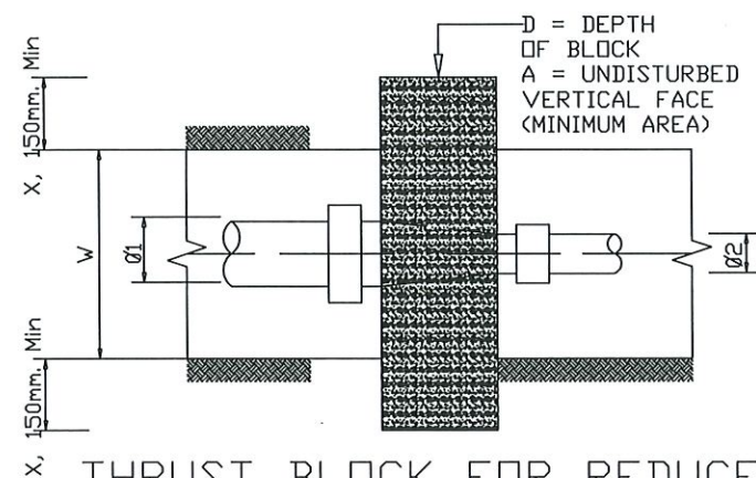
THRUST BLOCK FOR REDUCER
