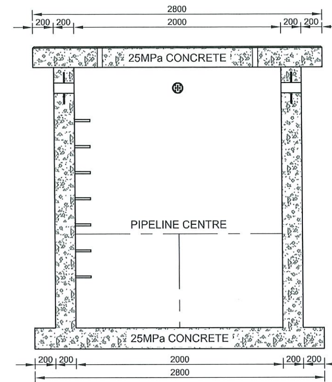
VALVE CHAMBER TYPICAL SECTION
