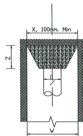
THRUST BLOCK FOR END CUP
