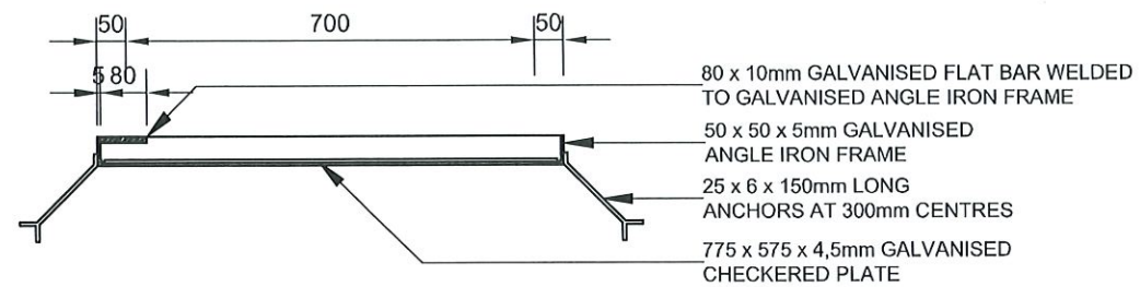
MANHOLE COVER SECTION
