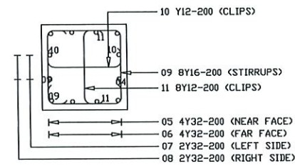
SECTION OF COLUMN SCALE 1:20
