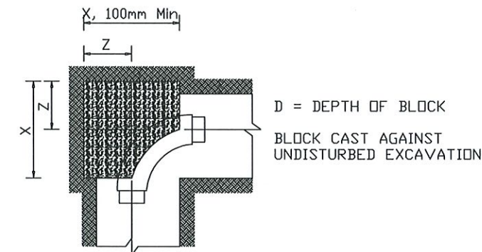
THRUST BLOCK FOR 90° BEND
