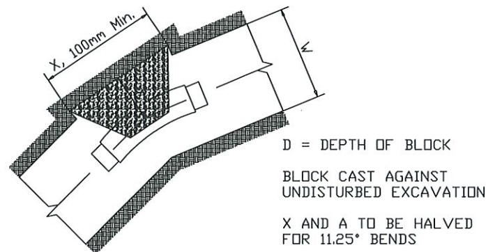
THRUST BLOCK FOR 22.5° & 11.25° BENDS
