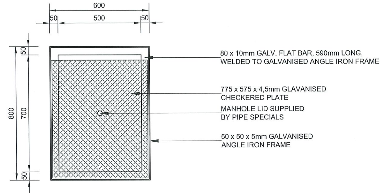
MANHOLE COVER PLAN
